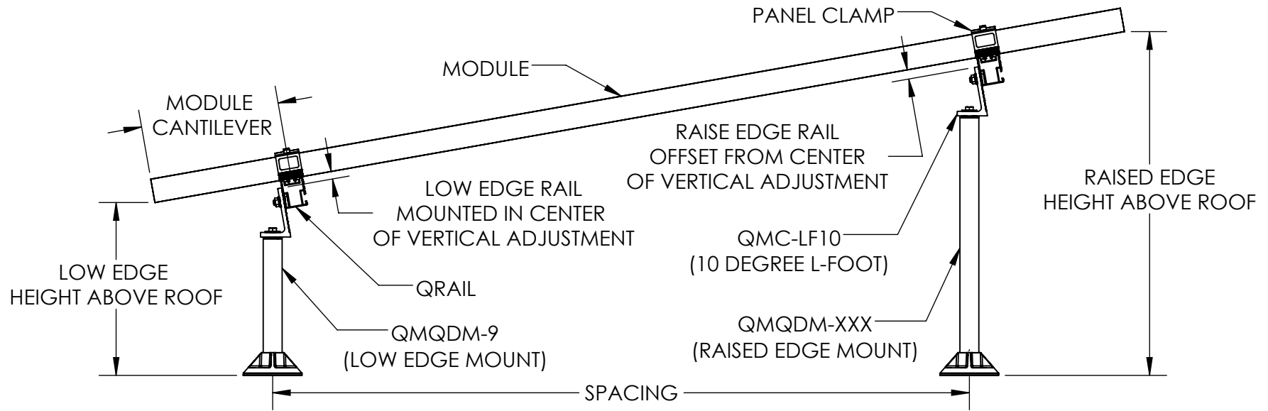
QRAIL TILT: QMADM-9 LOW EDGE MOUNT WITH 10 DEGREE TILT
